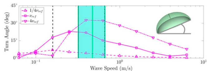
Fig. 7. Plot comparing the resulting turn angle of three bells with \nu = 1/4\nu_{ref} (dashed), \nu_{ref} (solid), and 4\nu_{ref} (dotted), at 2 s for differing activation wave speeds. We note that the peak turn angle is near the associated material wave speed (plotted in black). This suggests that this turning mechanism is strongly dependent on the interaction between the material properties of the bell and the speed of neuromuscular activation. Shaded in green is the range of speeds observed in A. aurita , with the solid green line representing the mean wave speed recorded.
