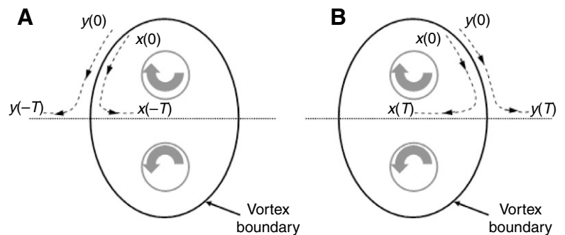
Fig. 2. A schematic drawing of a vortex boundary in a flow. Circles with inscribed arrows indicate vortex cores and their rotational sense. A pair of adjacent fluid particles close to but on different sides of the vortex boundary separate from each other faster than other arbitrary pairs of fluid particles, giving a larger value of the FTLE at the boundary. Trajectories can be followed in backward-time (A) to reveal attracting LCS, and in forward-time (B) to reveal repelling LCS boundaries.
